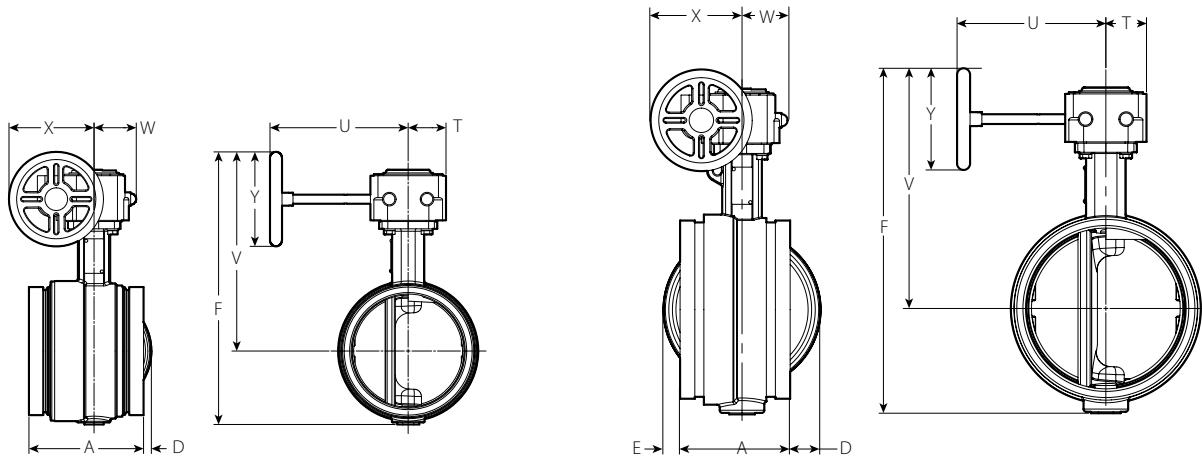
Gear Operator 2 – 6"/DN50 – 165.1 mm
