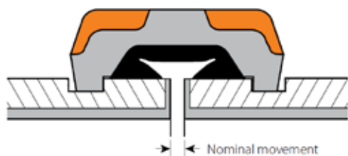
"PIPE-TO-PIPE" JOINT Refer to the table on the following page for the range of movement available
