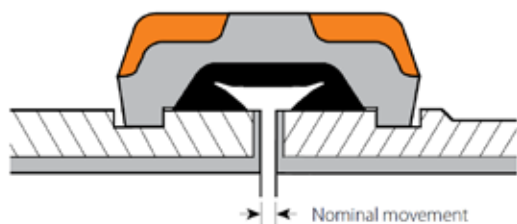
"PIPE-TO-FITTING" JOINT Refer to the table on the following page for the range of movement available
