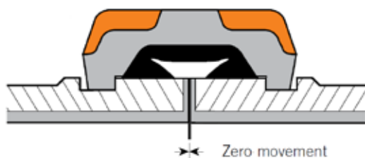
"FITTING-TO-FITTING" JOINT Fitting-to-Fitting joints do not include any separation or gap between the pipe ends and will not permit angular deflection or linear movement
