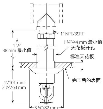
外伸裙座式带螺纹 V3613, V3615
