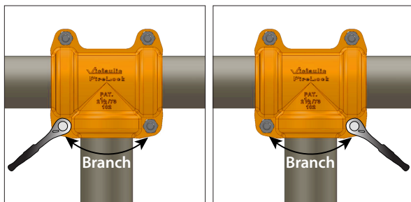
OVAL NECK OF BOLT SEATED PROPERLY
