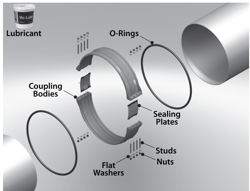
TYPE 2 COUPLING AND SEALING PLATES SHOWN
