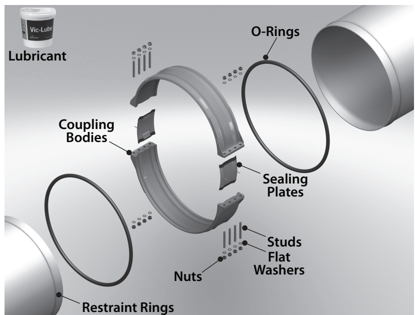
TYPE 2 COUPLING/SEALING PLATES SHOWN
