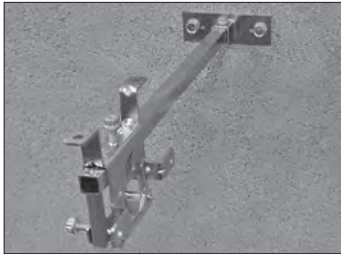
CANTILEVER MOUNT – SIDEWALL CONFIGURATION (FM)
