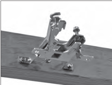
STANDOFF MOUNT – PENDENT CONFIGURATION (FM)
