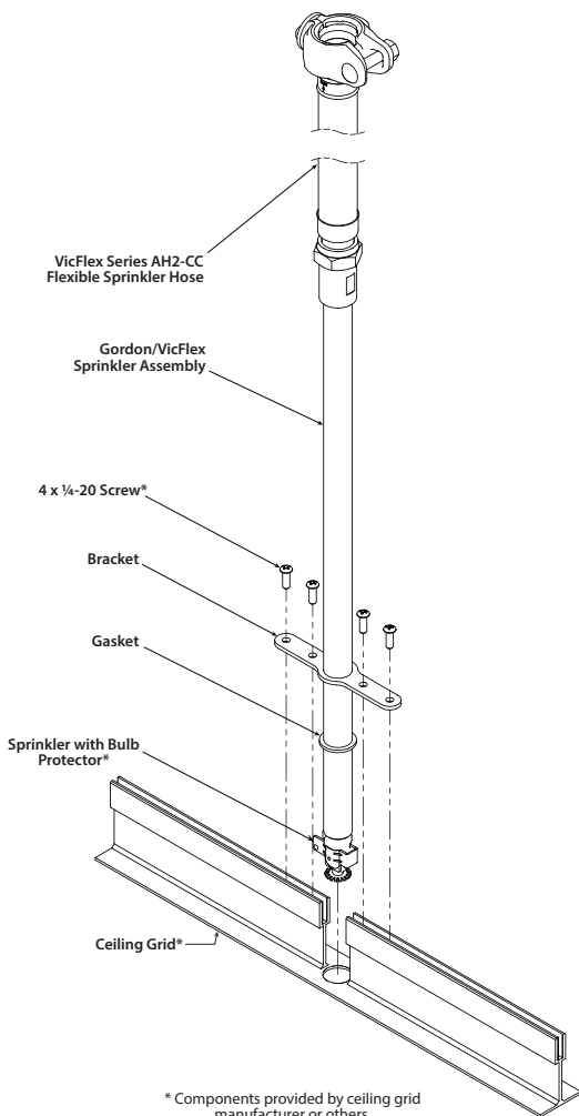
Exploded View of Installation Components
