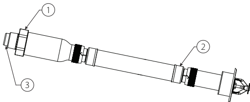
Recessed Pendent Shown Above
