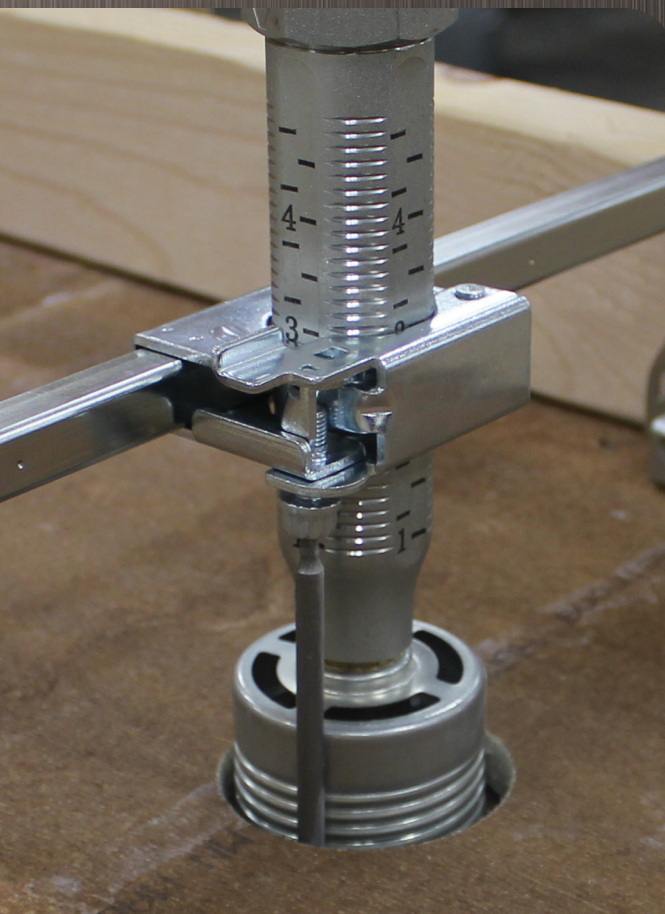
Loosen sprinkler/hose assembly in bracket with hand tool
