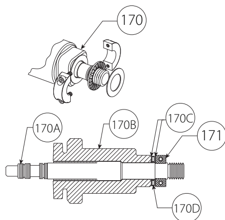
Arbor Assembly for ¾" Pipe (Item 170)
