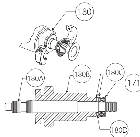
Arbor Assembly for 1 - 1½" Pipe (Item 180)
