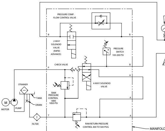
HYDRAULIC SCHEMATIC
